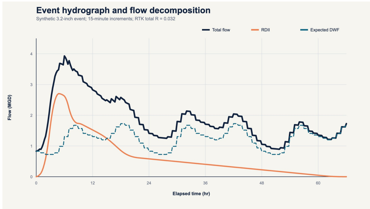
Event hydrograph
